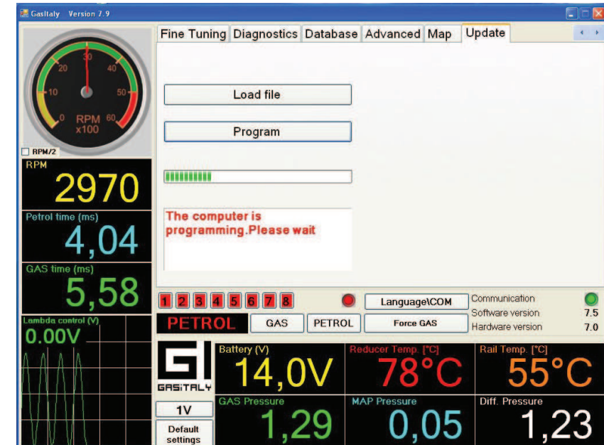
Pic. 13 UPDATE
