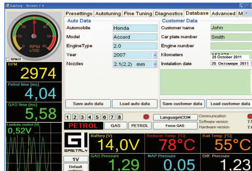
Pic. 6 Database
